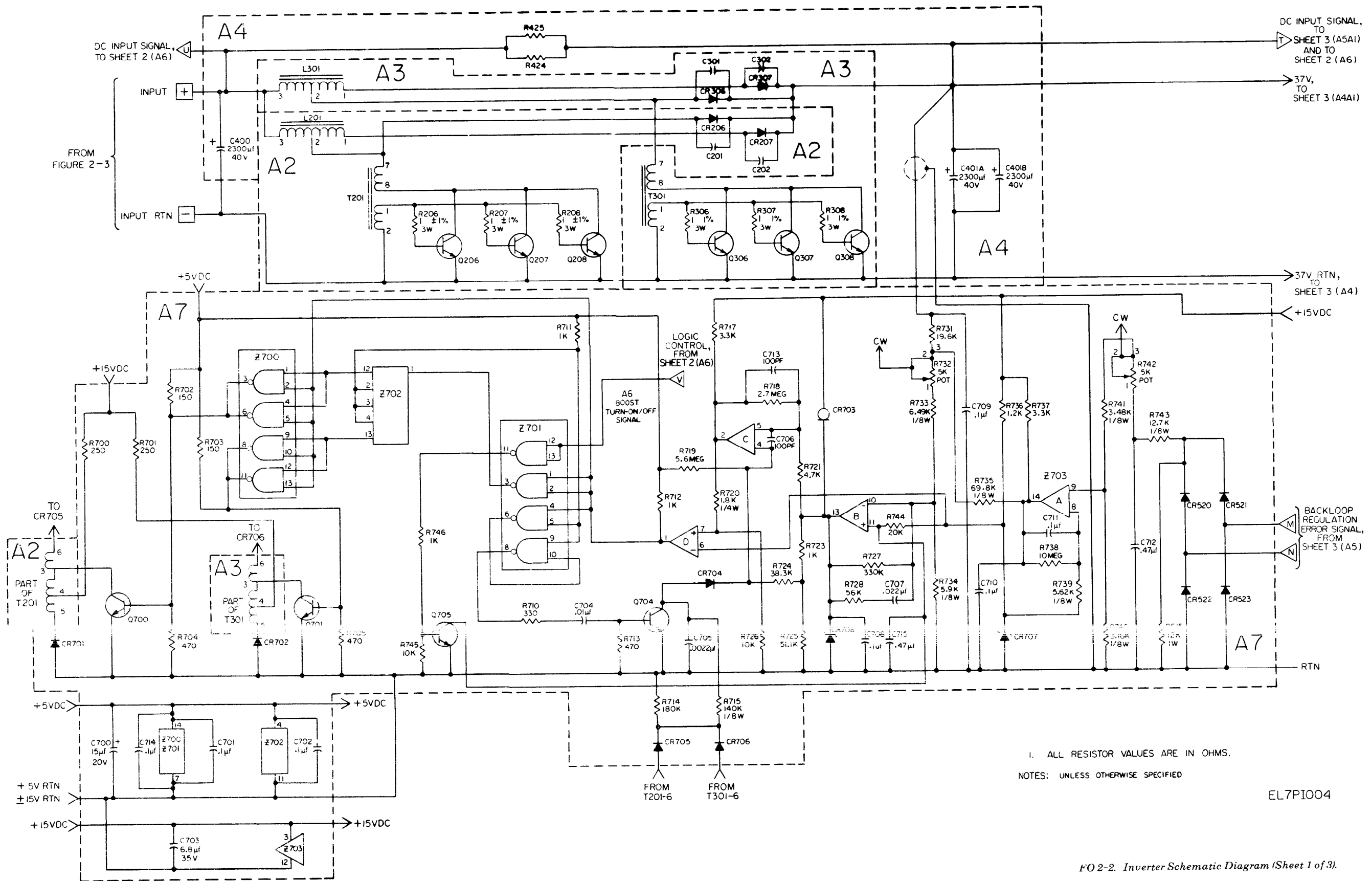
F02-2. Inverter Schematic Diagram (Sheet 1 of 3).
