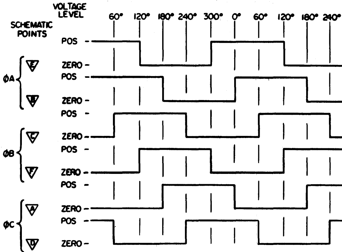
figure 2-4. Waveshape Inputs from Logic Ciccuits to Major Drive Section.
