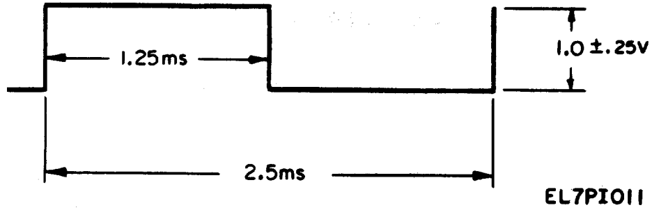
Figure 3-2. Input to Drivers of Major Bridge from Logic Assembly.
